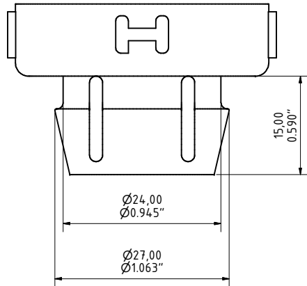
Clip-Stopfen III clip-in plug III I51000 Clip-Stopfen IV clip-in plug IV I4N000
